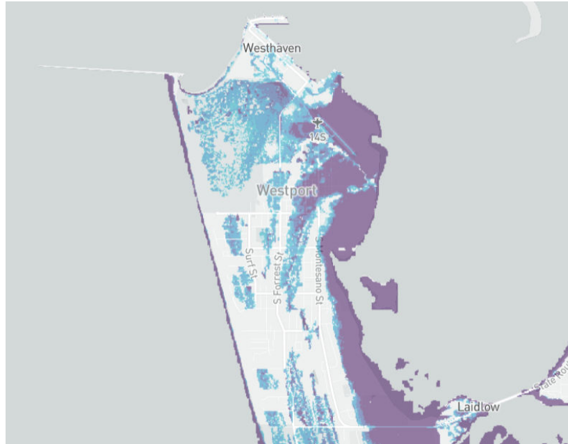
Fig 1. Map of Westport, Washington illustrating locations with a 0.2% chance of flooding this year. The shading indicates depth where the darkest purple displays roughly 3 ft deep flood water, and the lightest blue represents between 0 - 1 ft of flooding [Retrieved from: Flood Factor; 4].
